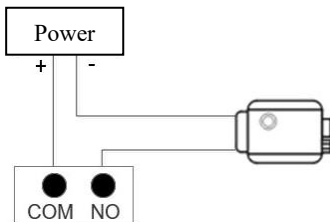
Normal open door lock wiring connection (door lock relay)
