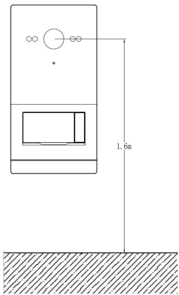
Suggested Installation Height: camera is 1.6m above the ground
