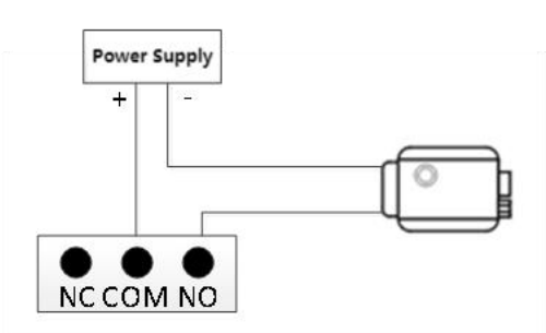
Wiring for normally open type lock(Electronic lock)
